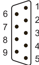
Stecker 9polig SubD
